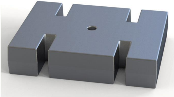
210x146x50mm 15kg Zwischenraum 16mm Loch 12mm Ref. CTP15.53
