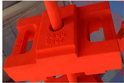
300x200x108mm 25kg Loch 33mm Ref. ST3378
