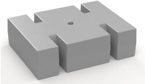
233x176x67mm 15.7kg Zwischenraum 16mm Loch 12mm Ref. M380002
