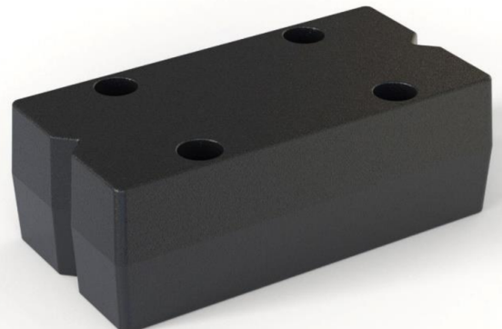
235x120x83mm 15.7kg Loch 20mm Ref. 15.7KG120
