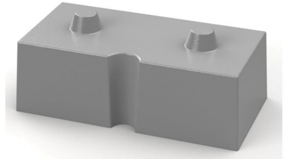
210x105x68mm 10kg Zwischenraum 11mm Ref. CP10KG68
