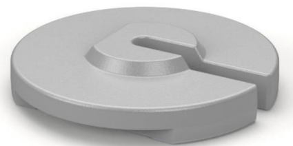
H: 44mm 20kg D: 310mm Ref: 7763
